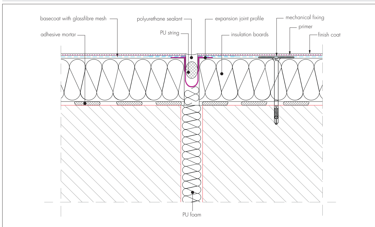
Figure 6 Vertical movement joint
