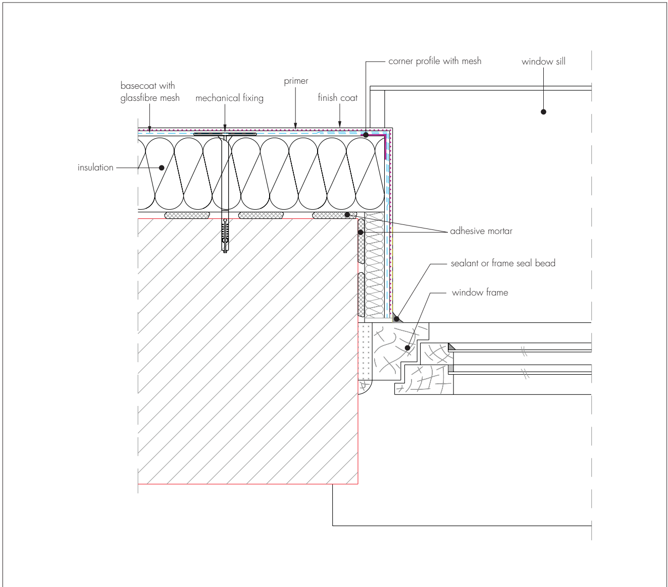
Figure 10 Insulated window reveal detail
