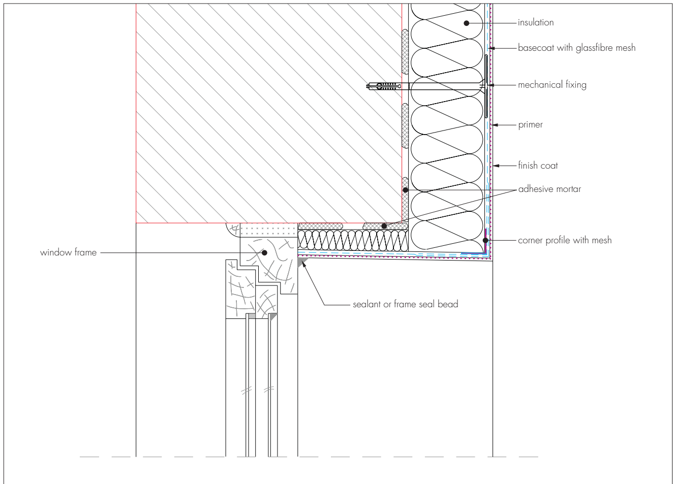
Figure 11 Insulated window head details
